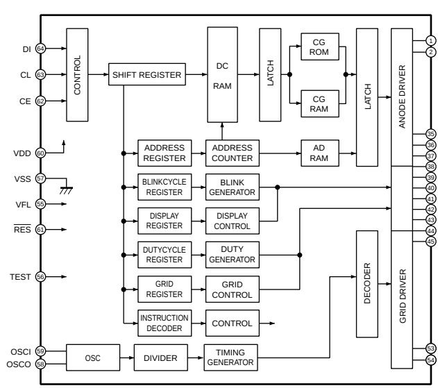
IC581: LC75712E FLD FL Display Driver
